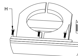
DETAIL C SCALE 1:10
