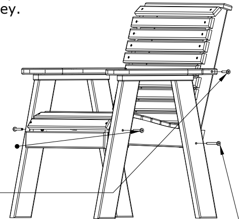
2 1/2" Stainless Wafer Bolt
